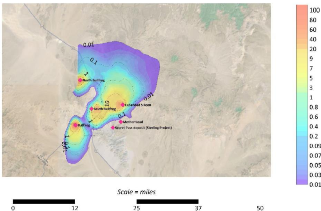
Figure 14. Drawdown scenario with 2,500 acre-feet of pumping. This is Scenario 2 from Roux 2024 (p. 5) (Appendix B) depicting cumulative drawdown in Oasis Valley due to pumping from four mines. Widespread drawdown of 5-10 feet is observable along the length of the Amargosa River. Actual pumping from these mines will be much higher.
