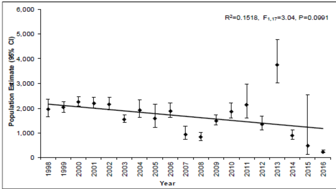
Figure 8. Amargosa toad robust design population model for all parcels combined from 1998 to 2016. Error bars depict the 95% confidence intervals (Kegerries et al. 2019, p. 19).
