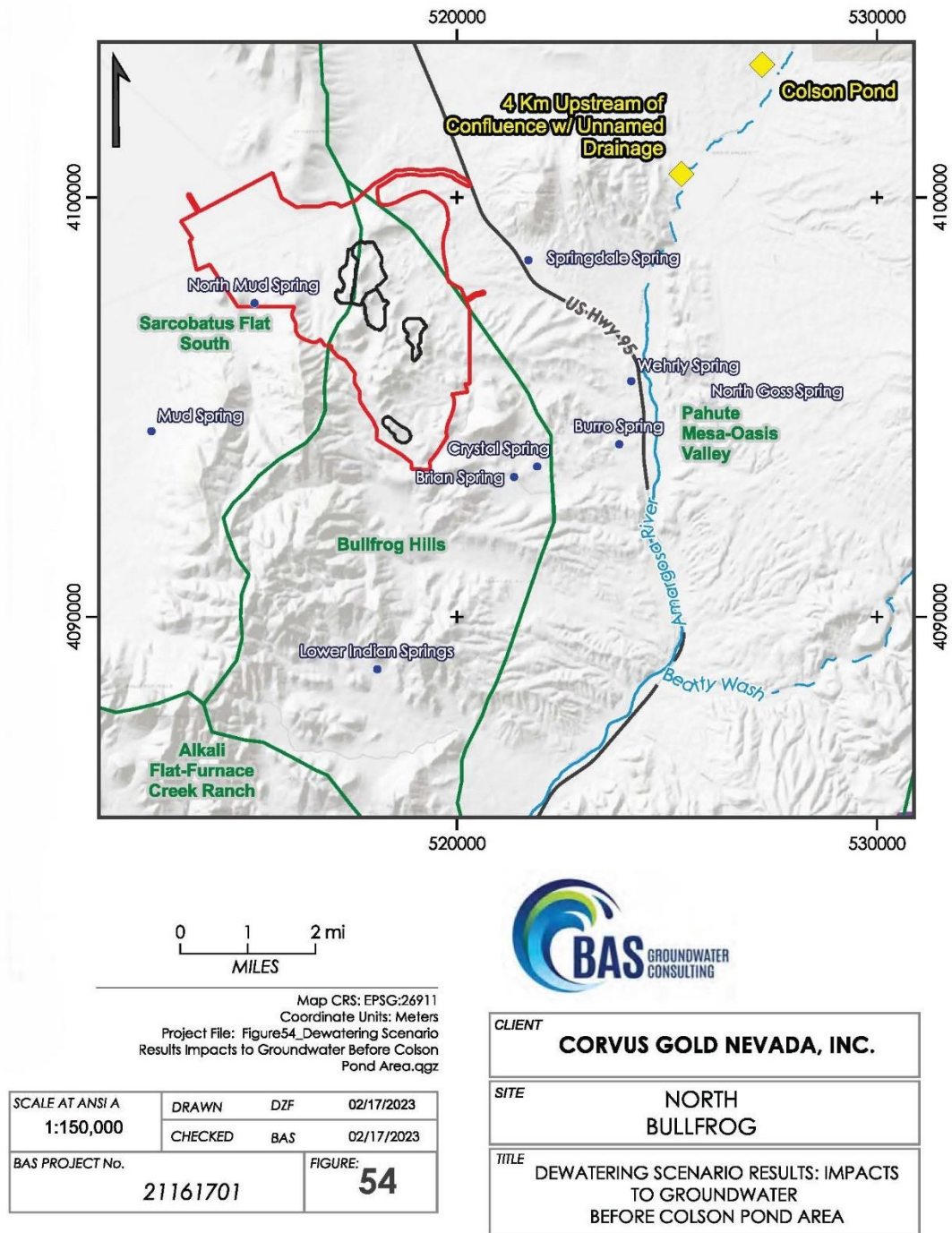
Figure 19. Location of the approximately 3.3 ft drawdown location along the Amargosa River 4 km upstream from the confluence with the unnamed drainage south of Springdale Spring. Also shown is Colson Pond. Adapted from HydroGeoLogica 2023, p. 656.
