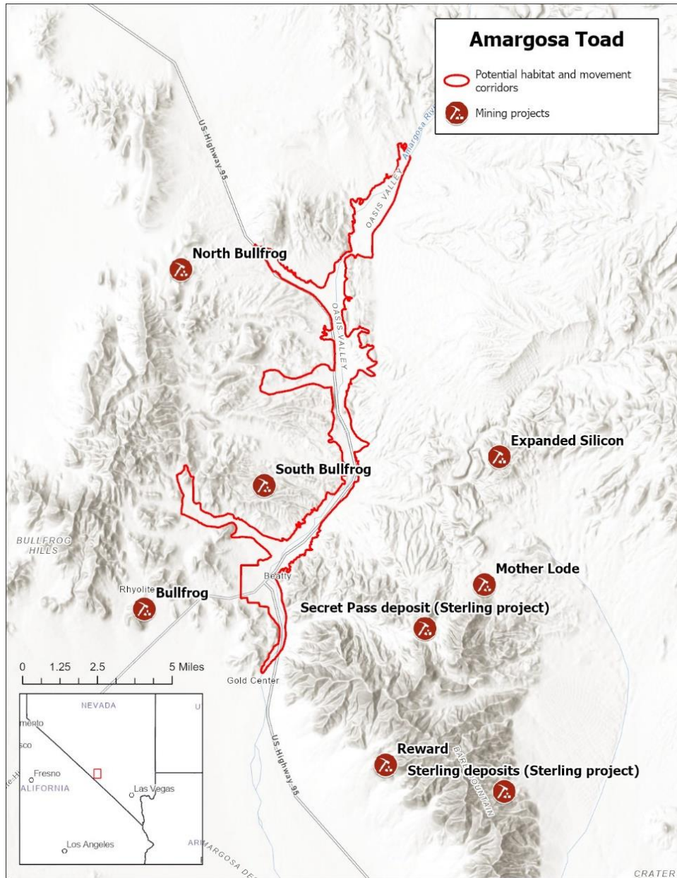
Figure 11. Map of Amargosa toad habitat and Beatty district gold mining projects. The location of the projects is approximate and based on the following sources: (a) North Bullfrog (AngloGold Ashanti 2022, p. 197); (b) South Bullfrog (Zacapa Resources 2021, p. 1); (c) Bullfrog (Augusta Gold 2022a, p. 159); (d) Expanded Silicon (AngloGold Ashanti 2022, p. 201, 203); (e) Mother Lode (AngloGold Ashanti 2022, p. 210); (f) Reward (Augusta Gold 2022a, p. 15, 159); (g) Sterling (AngloGold Ashanti 2022, p. 210). The Sterling project is represented as two separate projects, “Secret Pass deposit (Sterling project)” and “Sterling deposits (Sterling project)” as individual deposits are spread over a distance of approximately 10 km and it seems likely that more than one mine could be built.
