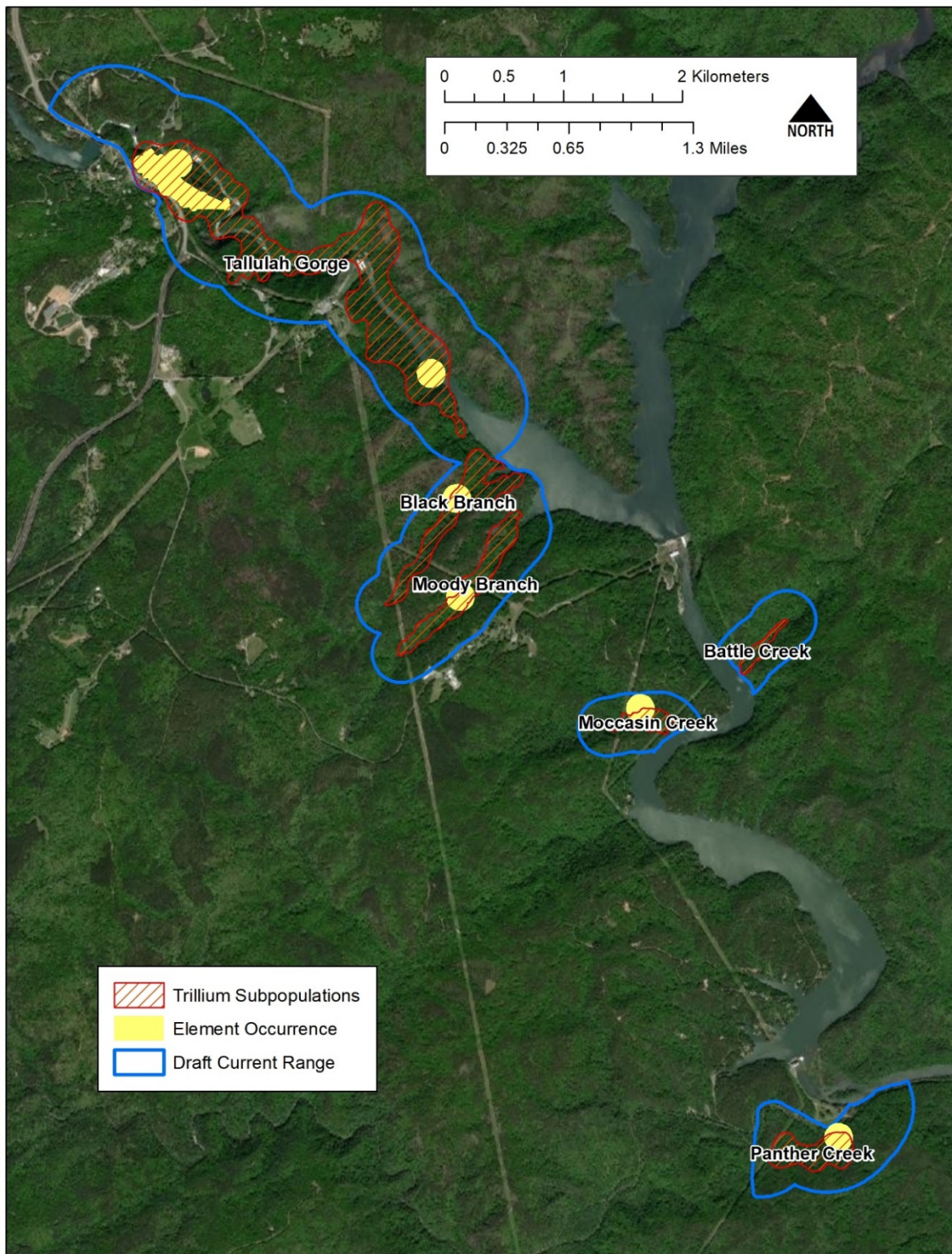
Figure 2. Draft current range for Trillium persistens sub-populations across the Tallulah River drainage in Georgia and South Carolina. Populations as reported in the recovery plan include the Tallulah River (including Tallulah Gorge, Black Branch and Moody Branch subpopulations), Battle Creek, Moccasin Creek, and Panther Creek (USFWS 1984).
