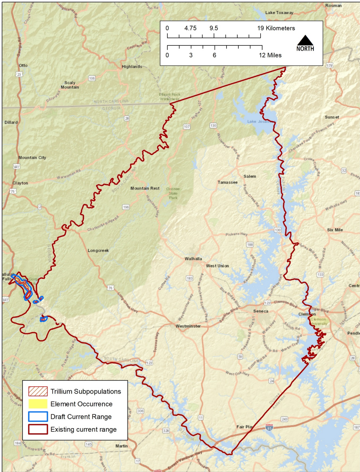
Figure 1. Range of Trillium persistens across Georgia and South Carolina.
